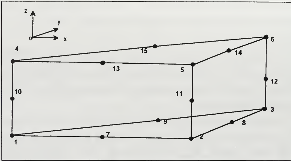
Figure 3. PRIS15F Element Topology. After Ref.[3]
